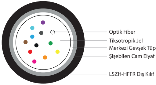
12 Fiber 1x12
