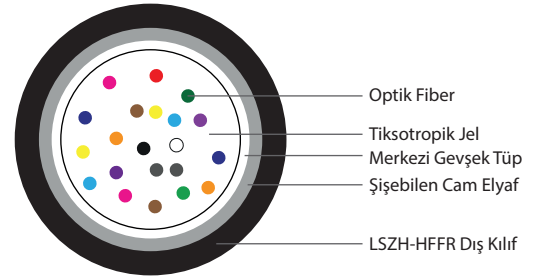
24 Fiber 1x24
