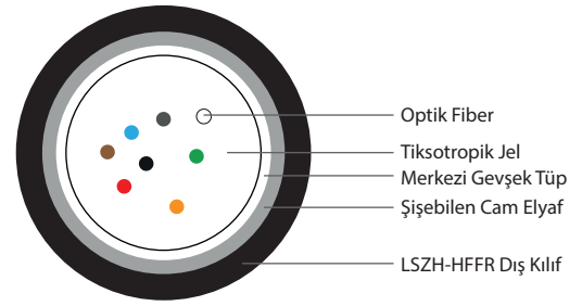
24 Fiber 1x24
