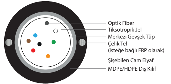
24 Fiber 1x24
