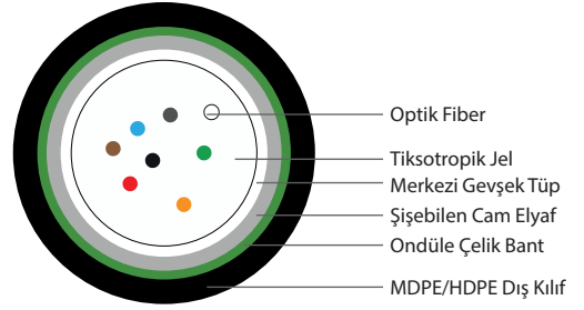
24 Fiber 1x24
