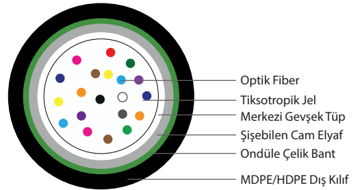
24 Fiber 1x24
