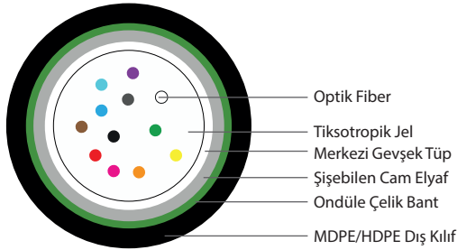
12 Fiber 1x12
