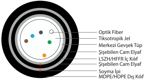
12 Fiber 1x12
