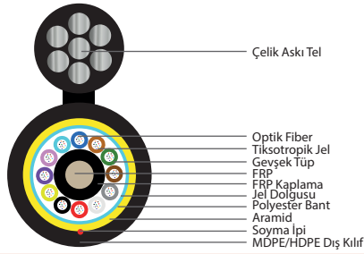
144 Fiber 12x12
