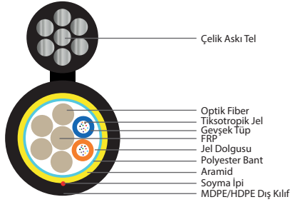
48 Fiber 4x12
