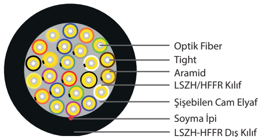
24 Fiber
